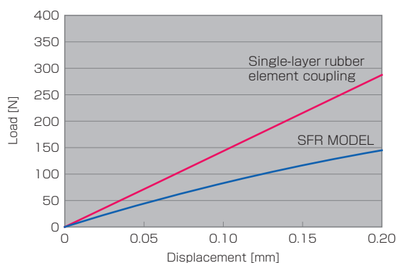
Comparison of counterforces for parallel misalignment
