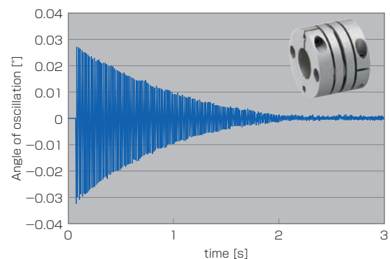
Metal disk coupling
