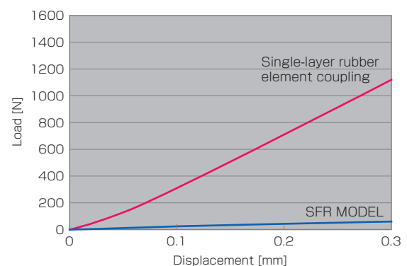
Comparison of counterforces along the axial direction
