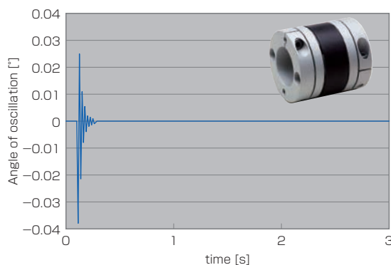
High-damping rubber element coupling
